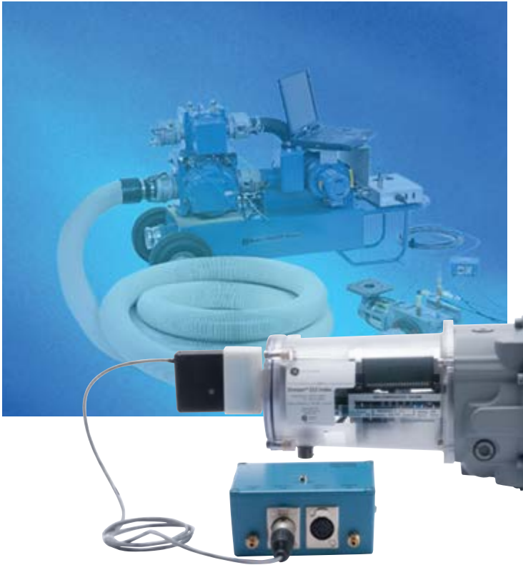
ES3 Prover Cable to Model 5 Prover Field Junction Box
